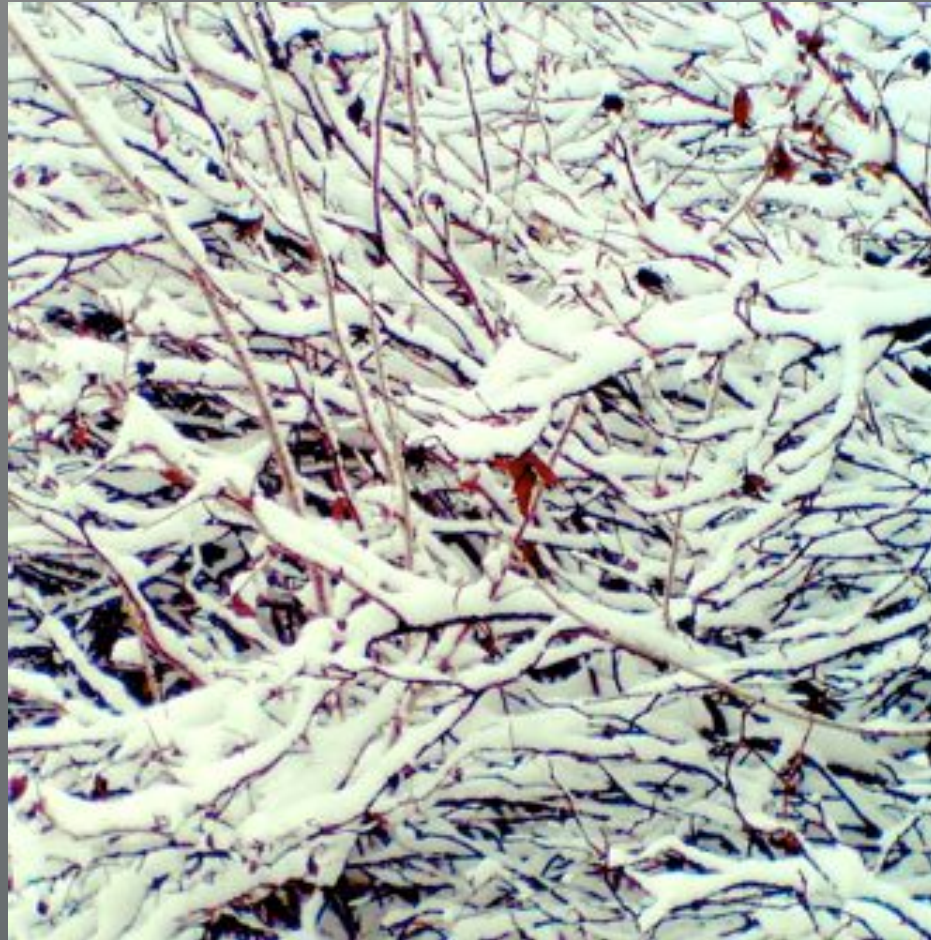
Snow covered branches – Mátra - Hungary
